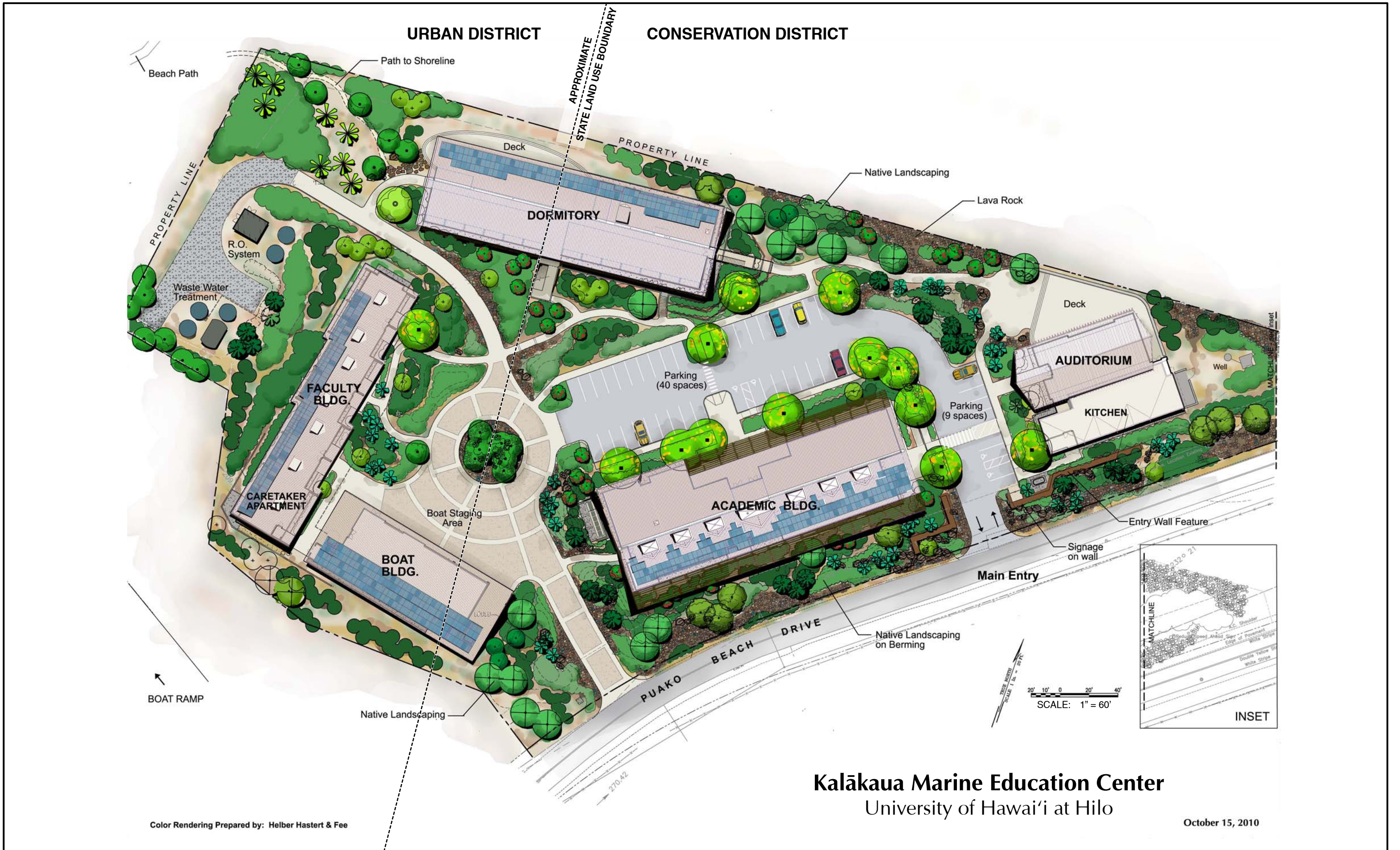
Figure 4: Schematic Site Plan
